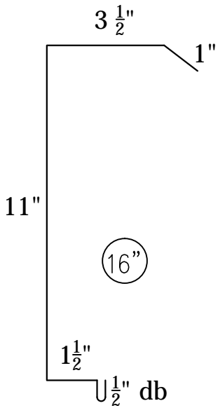
1 PIECE GABLE FASCIA
