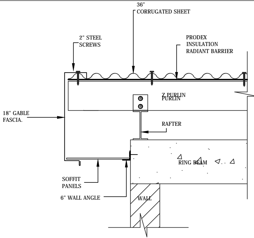
GABLE FASCIA DETAIL
