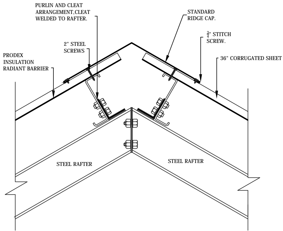
RIDGE CAP & HIP DETAIL
