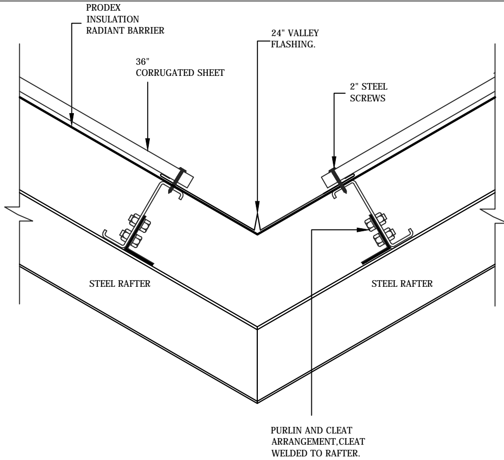
VALLEY TRIM DETAIL
