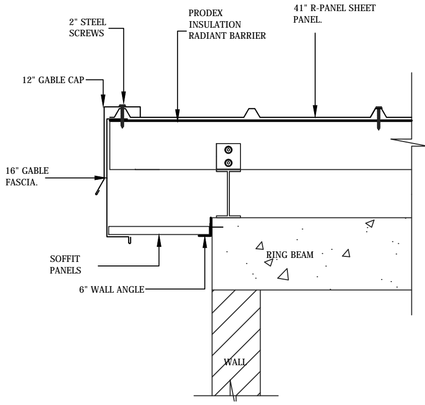
GABLE FASCIA AND GABLE CAP DETAIL
