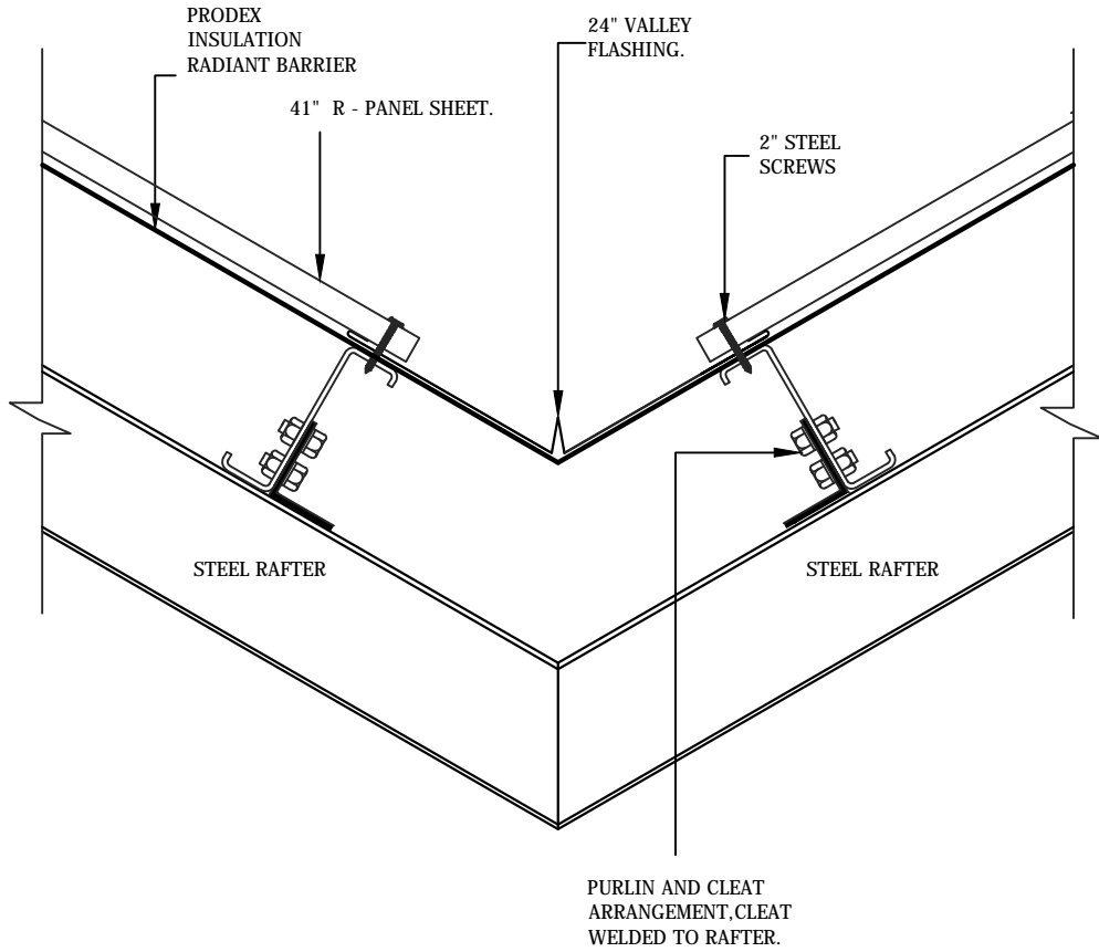
VALLEY TRIM DETAIL
