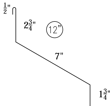
HEAD WALL
