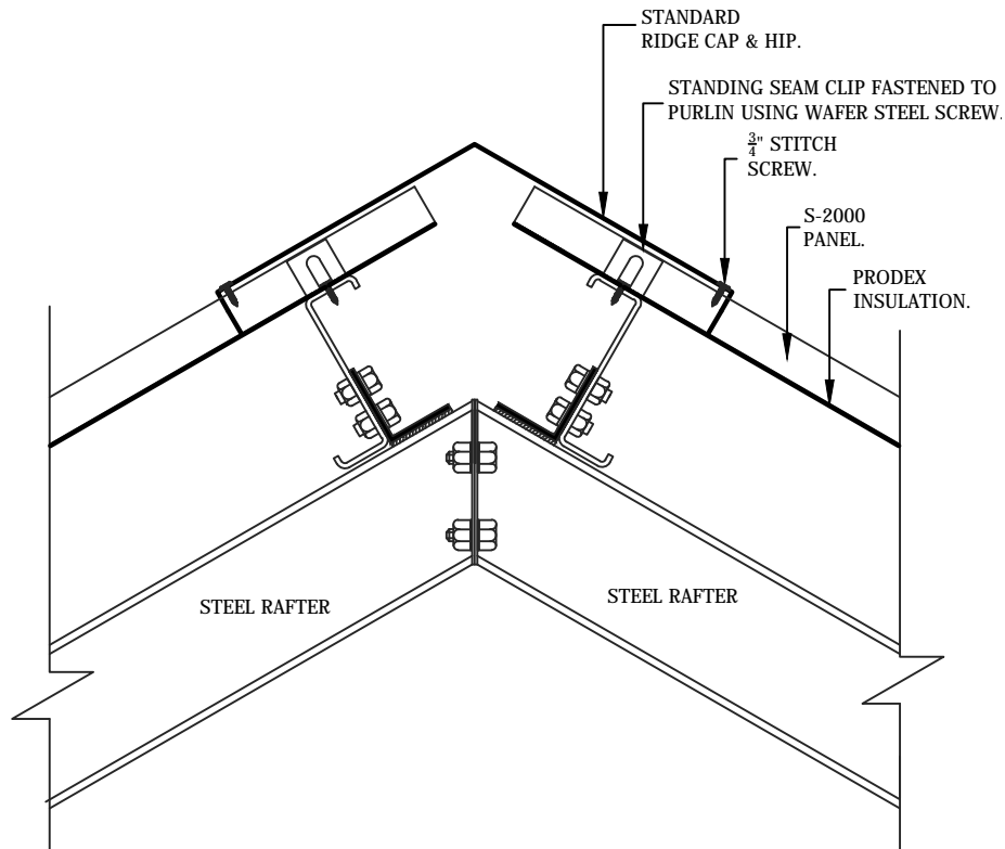
RIDGE CAP & HIP DETAIL
