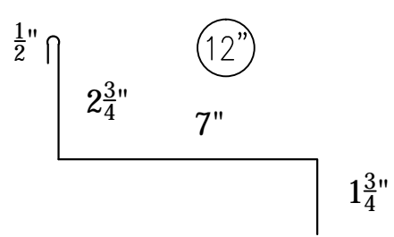
SIDE WALL
