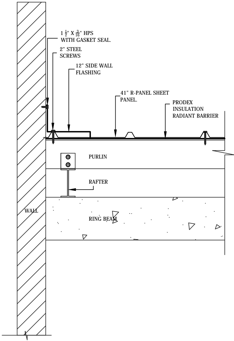
SIDE WALL DETAIL
