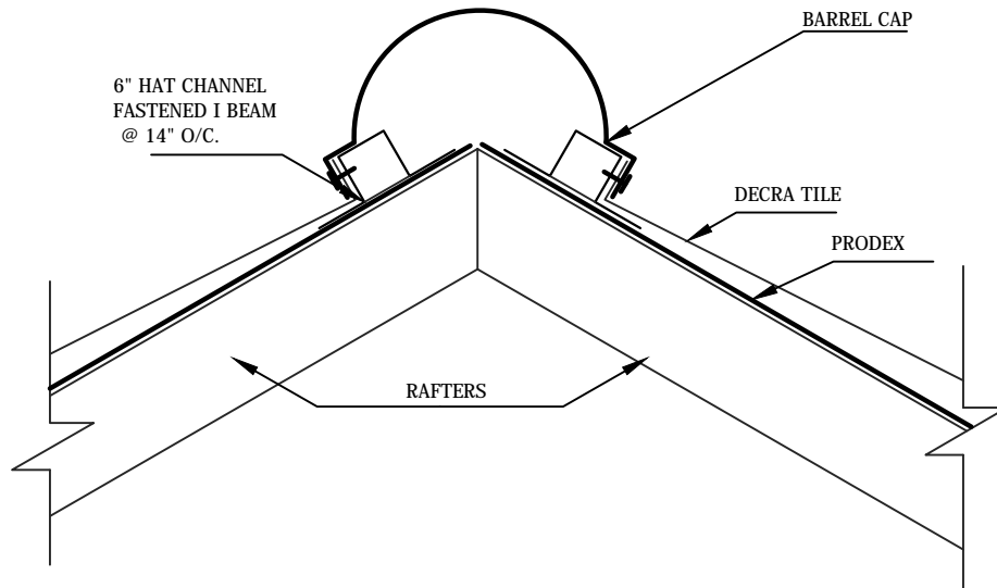
○ DECRA-EAVE DETAIL Scale:
