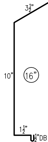
EAVE FASCIA
