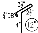
STARTER TRIM
