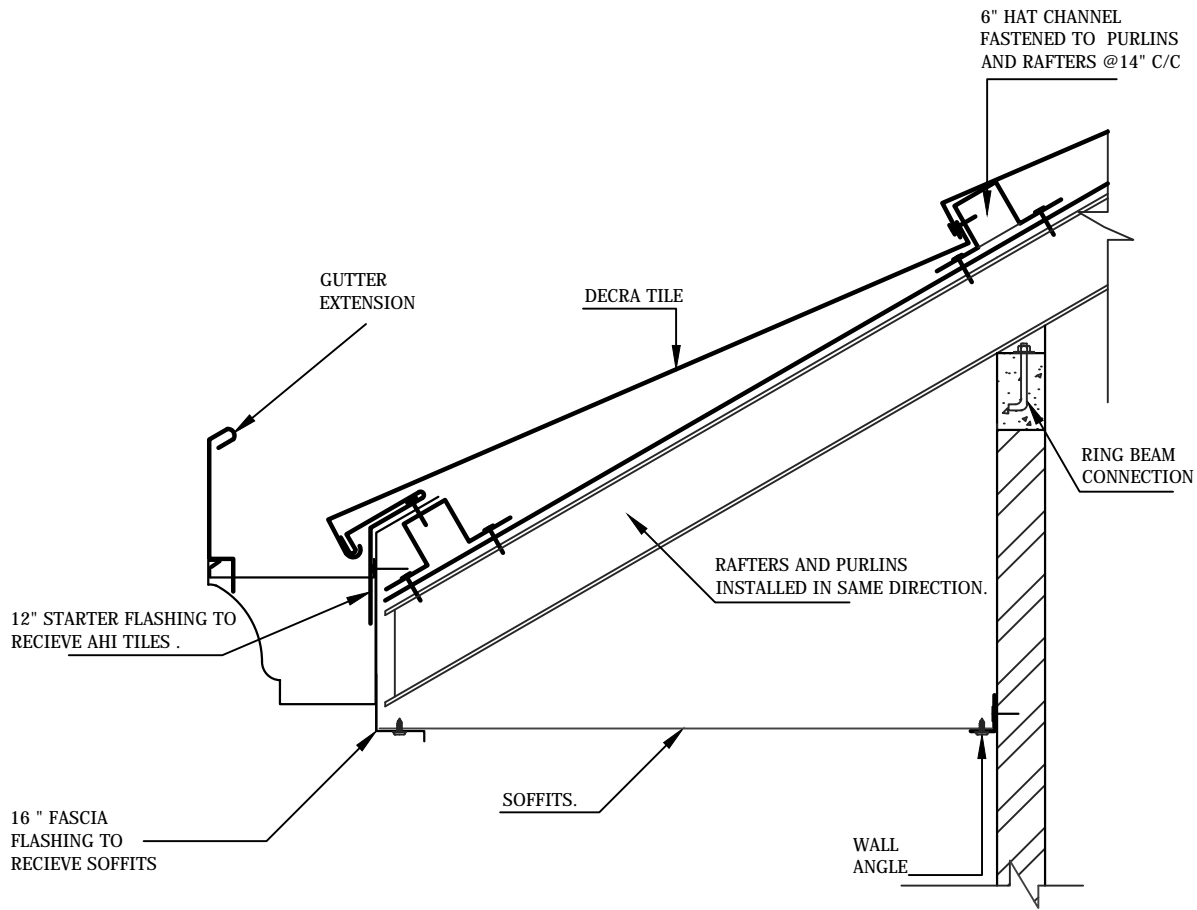
○ DECRA-EAVE DETAIL Scale:
