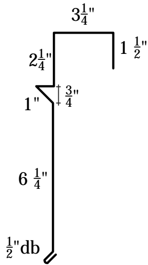
GABLE FASCIA
