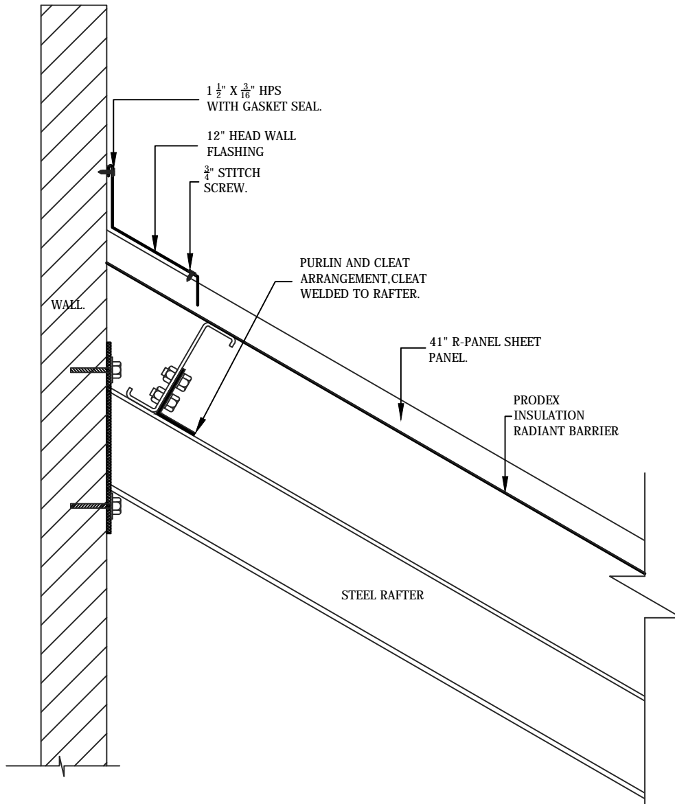
HEAD WALL DETAIL
